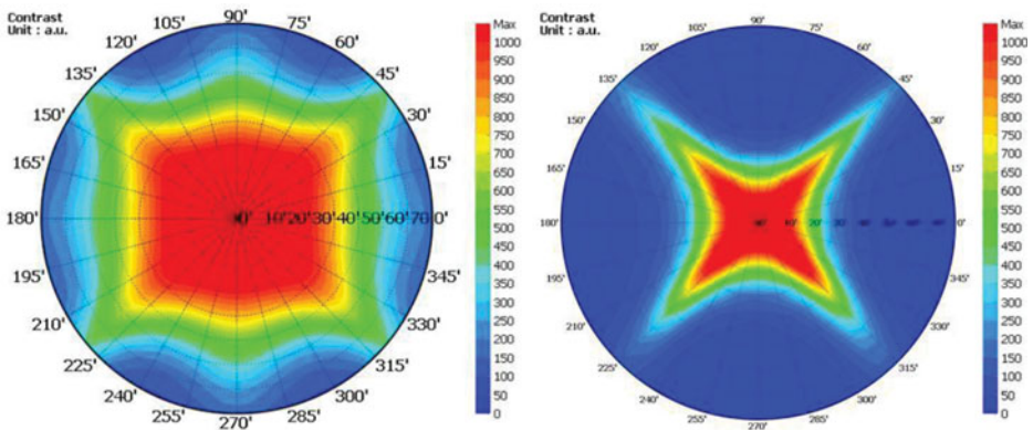
Figure 6. The calculated iso-contrast contour of (a) the MVA LC mode and (b) WV-TN mode.
